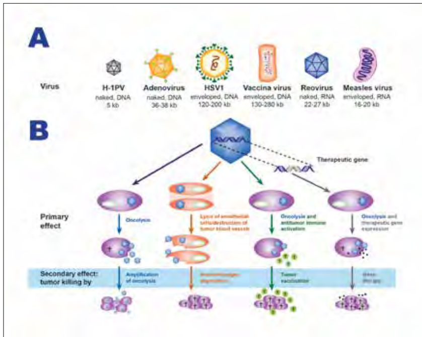
Figure 1: A. Different families of viruses that can have oncolytic effects upon cancer cells. B. Varying mechanisms of action that viruses can employ to kill cancer cells.
